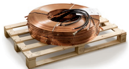
Conductor strip package ready for assembly
